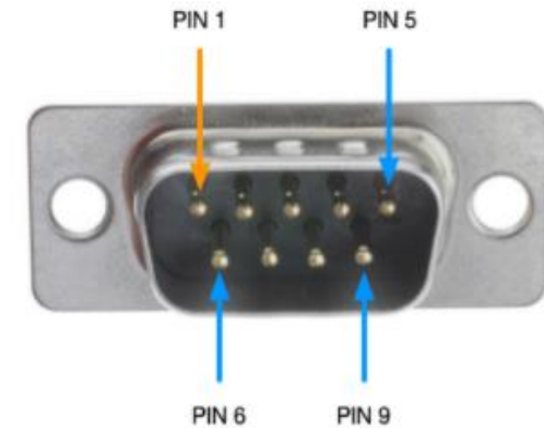
Conector DB9 Male
